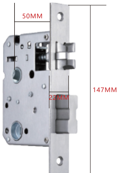
B1 lock body (center distance 50MM)
