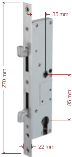
6 # (double hook 35 * 85 + without locks)
