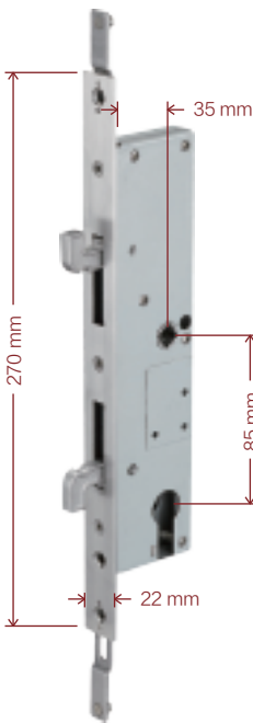
6 # (double hook 35 * 85 + lockwith heaven and earth)
