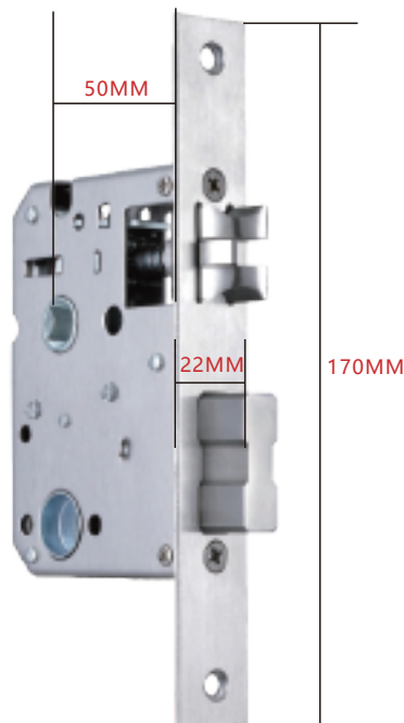
B2 lock body (center distance 50MM)
